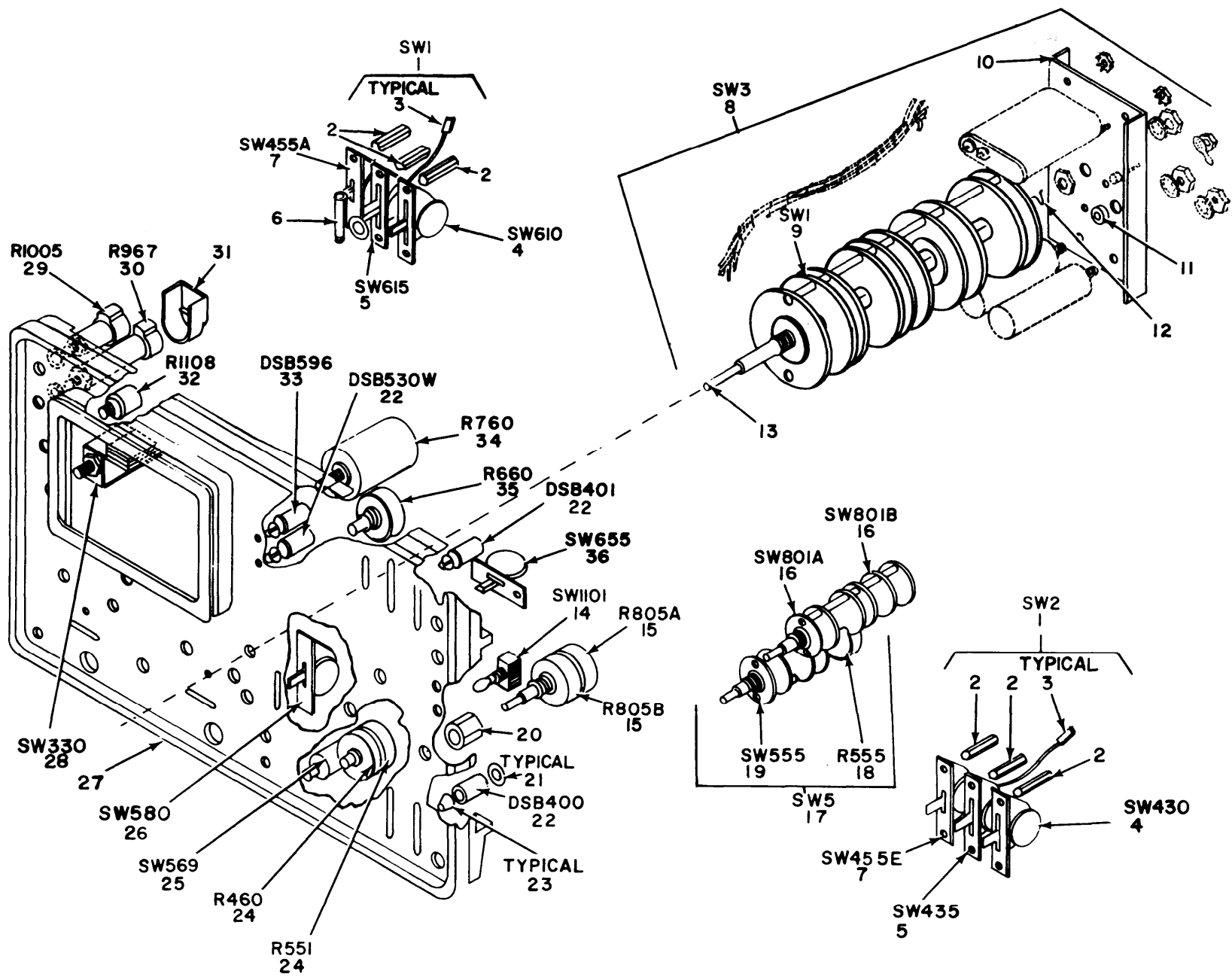
Figure 11. Oscilloscope AN/USM-273, Electronic Components Location.
