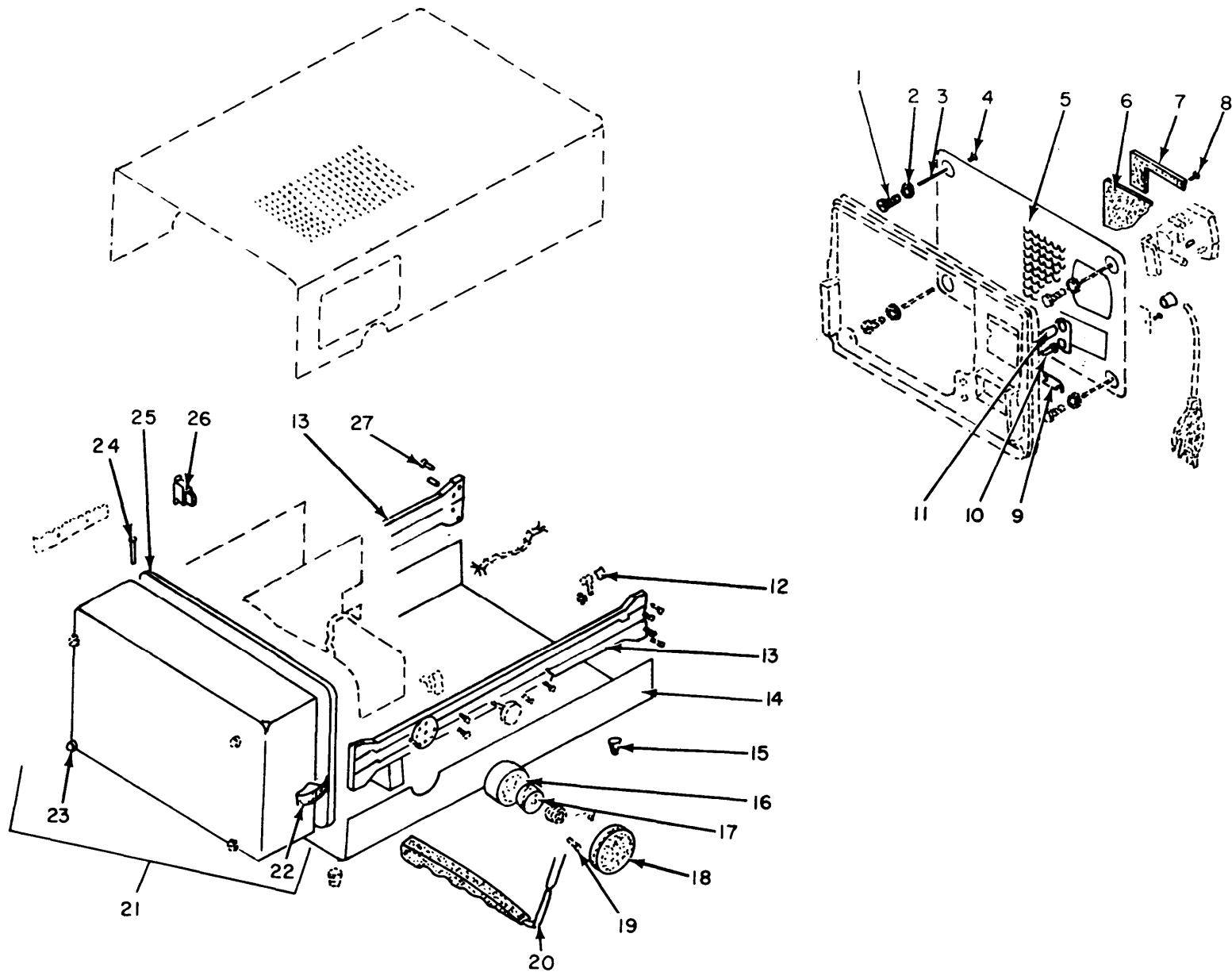
Figure 16. Oscilloscope AN/USM-273, Frame and Cabinet (Sheet 1 of 5).
