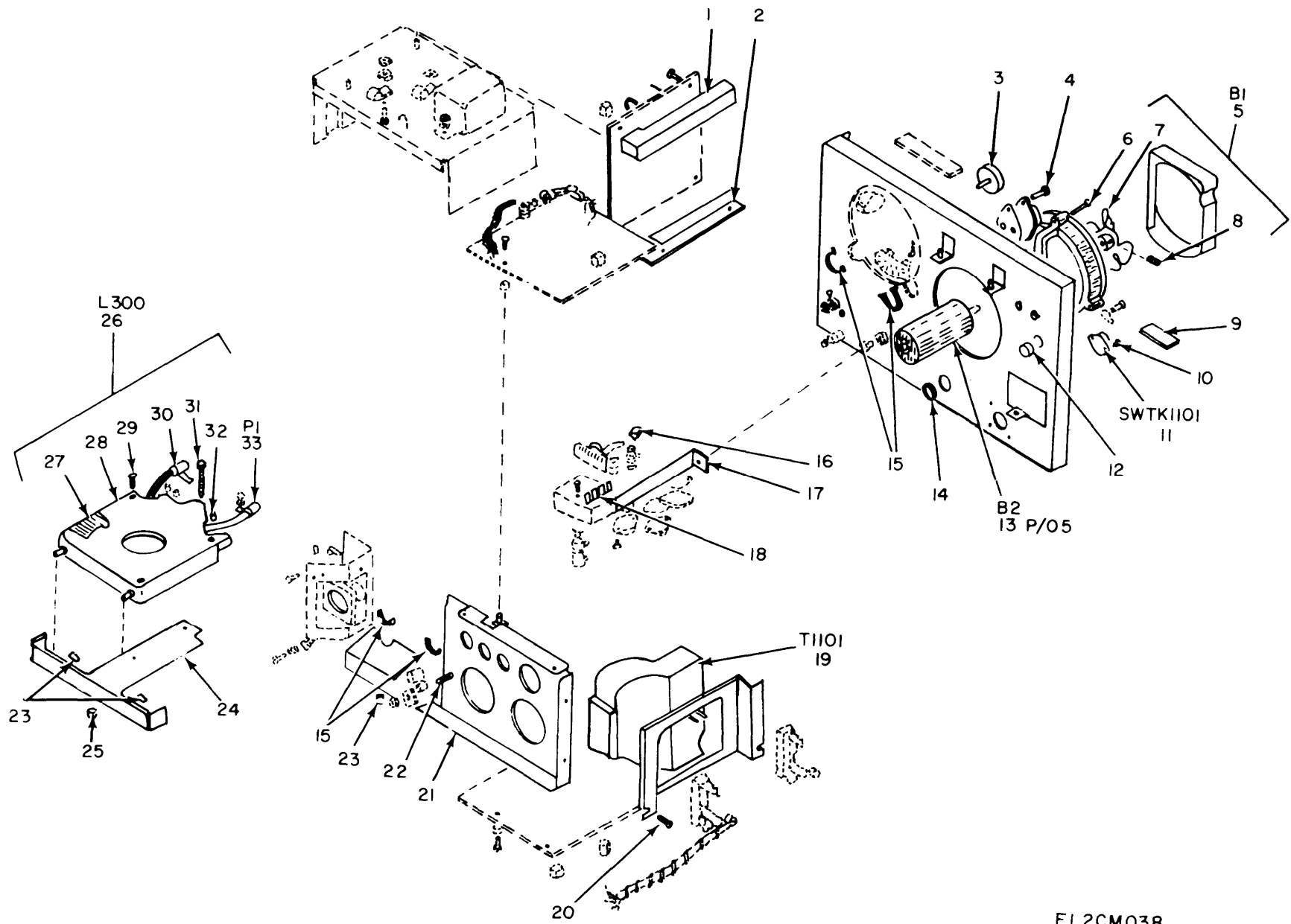
Figure 15. Oscilloscope AN/USM-273, Rear Chassis.
