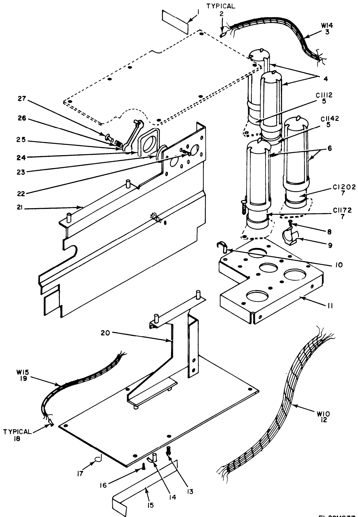
Figure 14. Oscilloscope AN/USM-273, A and B Sweeps.
