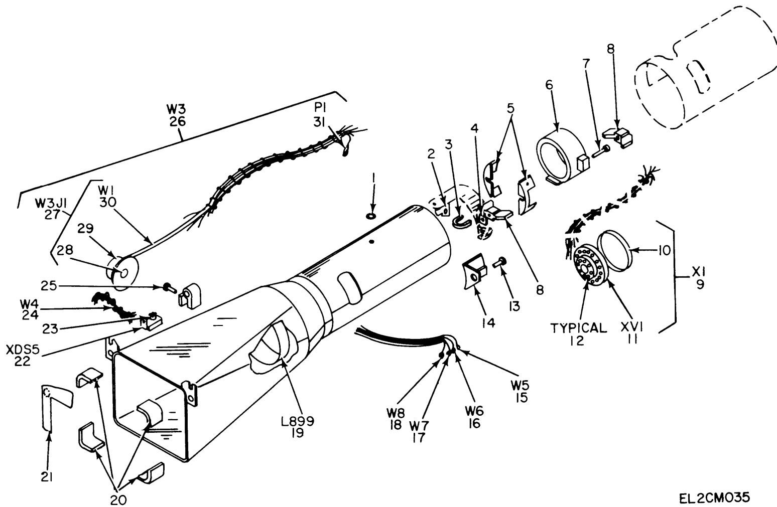
Figure 13. Oscilloscope AN/USM-273, CRT Shield (Sheet 1 of 2).
