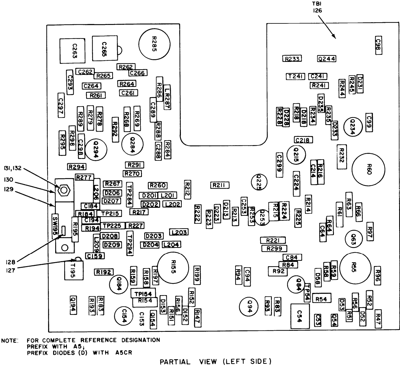
Figure 5. Oscilloscope AN/USM-273, Vertical Preamplifier Circuit Board (A5) (Sheet 1 of 6).
